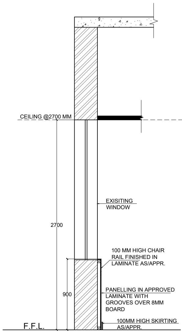
SECTION A
