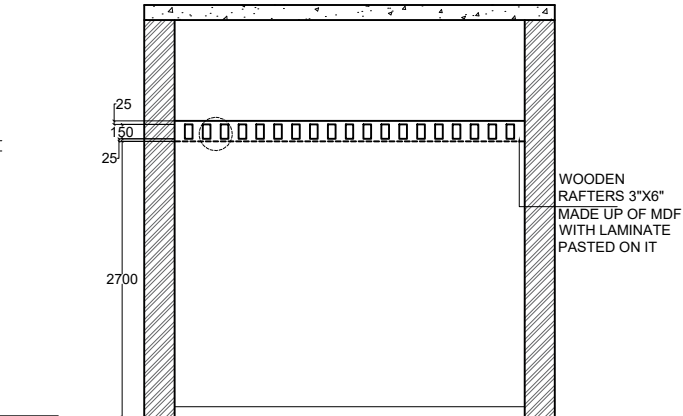
ELEVATION C
