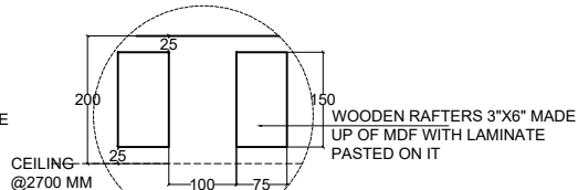
DETAIL Z
