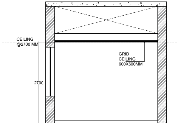
ELEVATION D
